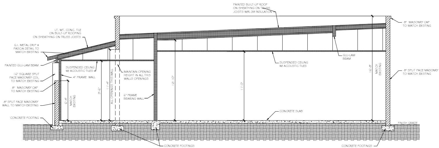
1 BUILDING SECTION 3/8" = 1'-0"
